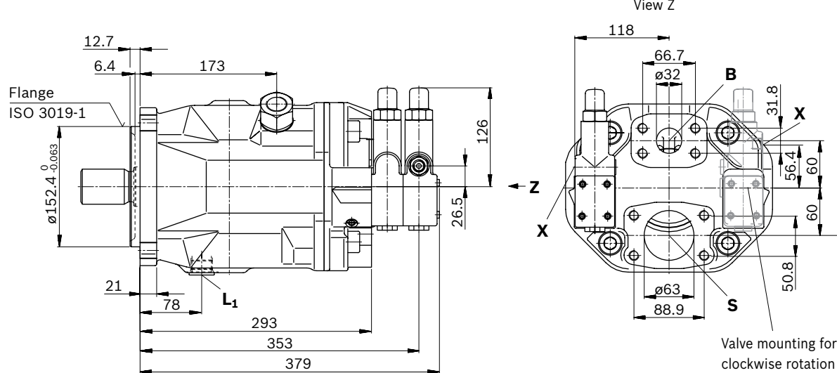
View Z
