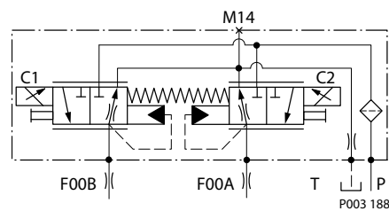
NFPE schematic
