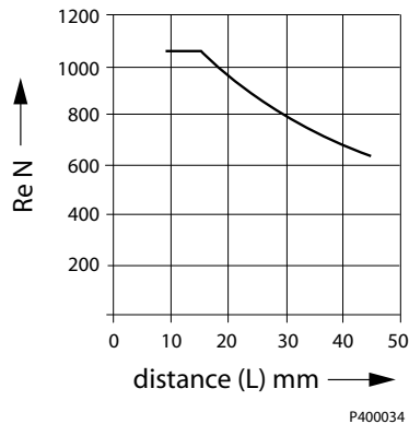
Maximum allowable radial load (Re)
