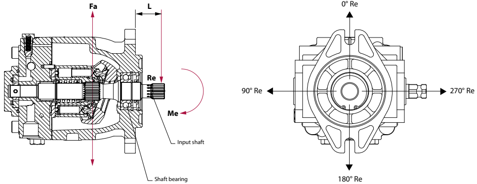
Maximum allowable radial load (Re)
