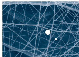
Enlarged Top Views of Media (at the same magnification.) White circles represent the diameter of a 2µ and a 5µ particle.
